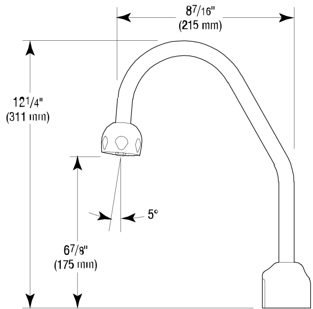
Variations not shown: Above Deck Mixer with 8" Trim Plate
